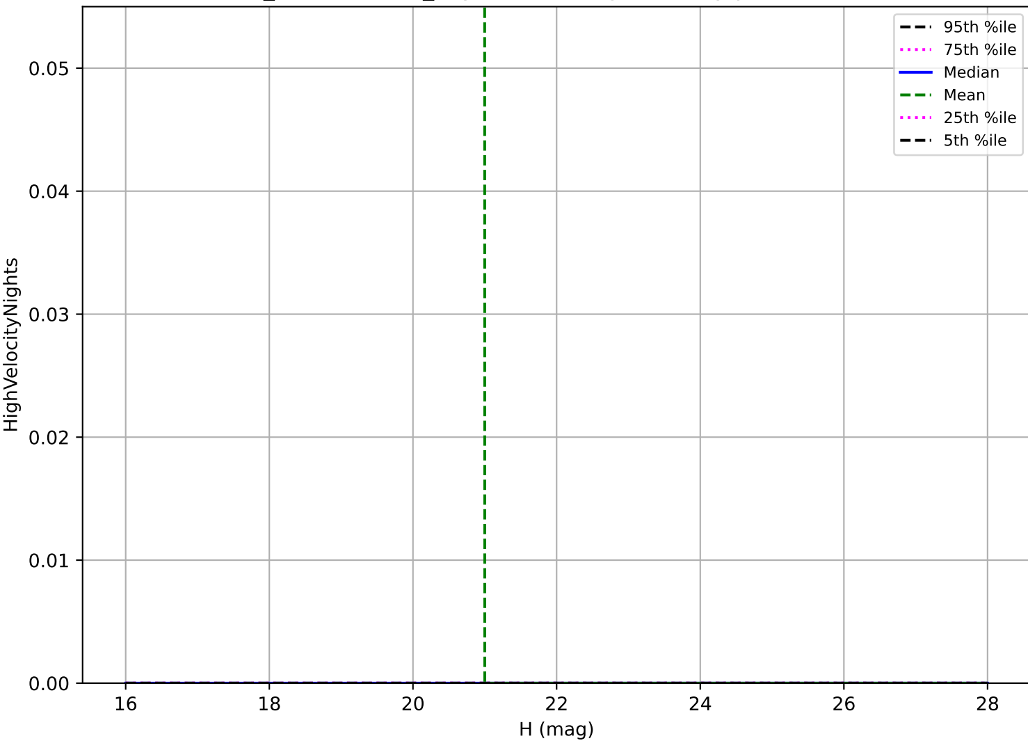
weather_cloudso4v3.4_10yrs: Vatira High velocity pair detection loss
