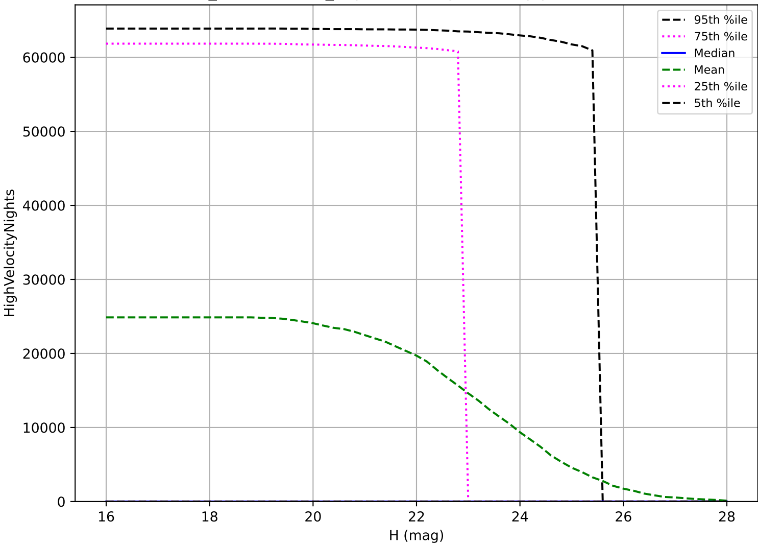
weather_cloudso4v3.4_10yrs: PHA High velocity pair detection loss
