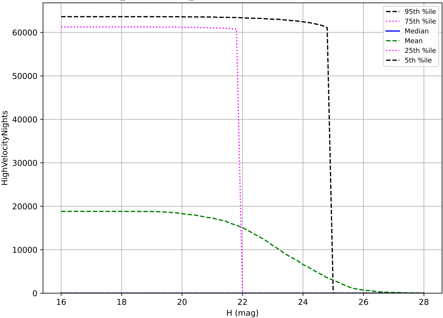
weather_cloudso4v3.4_10yrs: NEO High velocity pair detection loss
