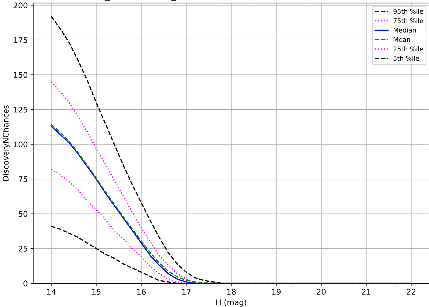
weather_cloudso4v3.4_10yrs: Trojan 3 pairs in 15 nights detection loss
