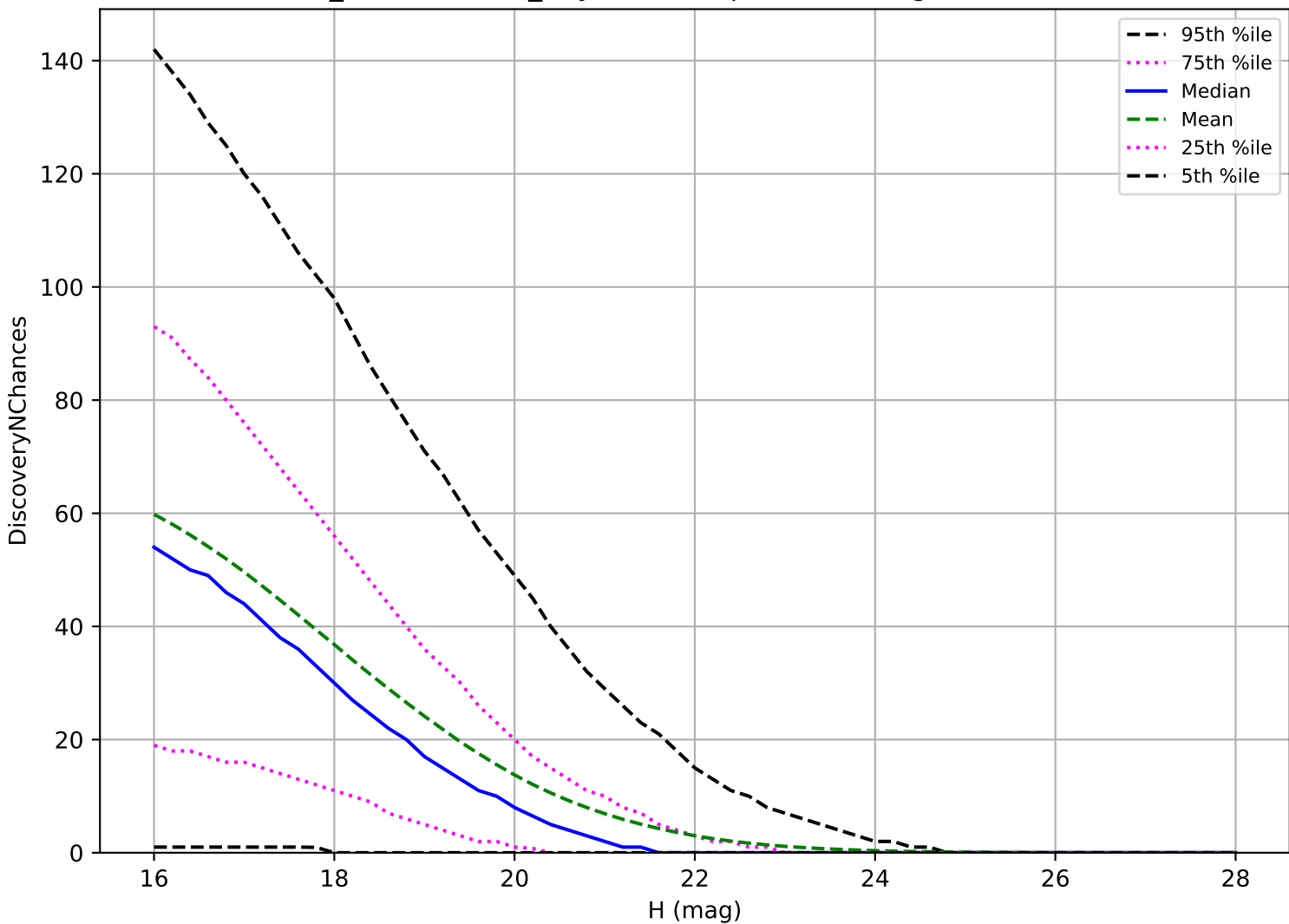
weather_cloudso4v3.4_10yrs: PHA 3 pairs in 15 nights detection loss
