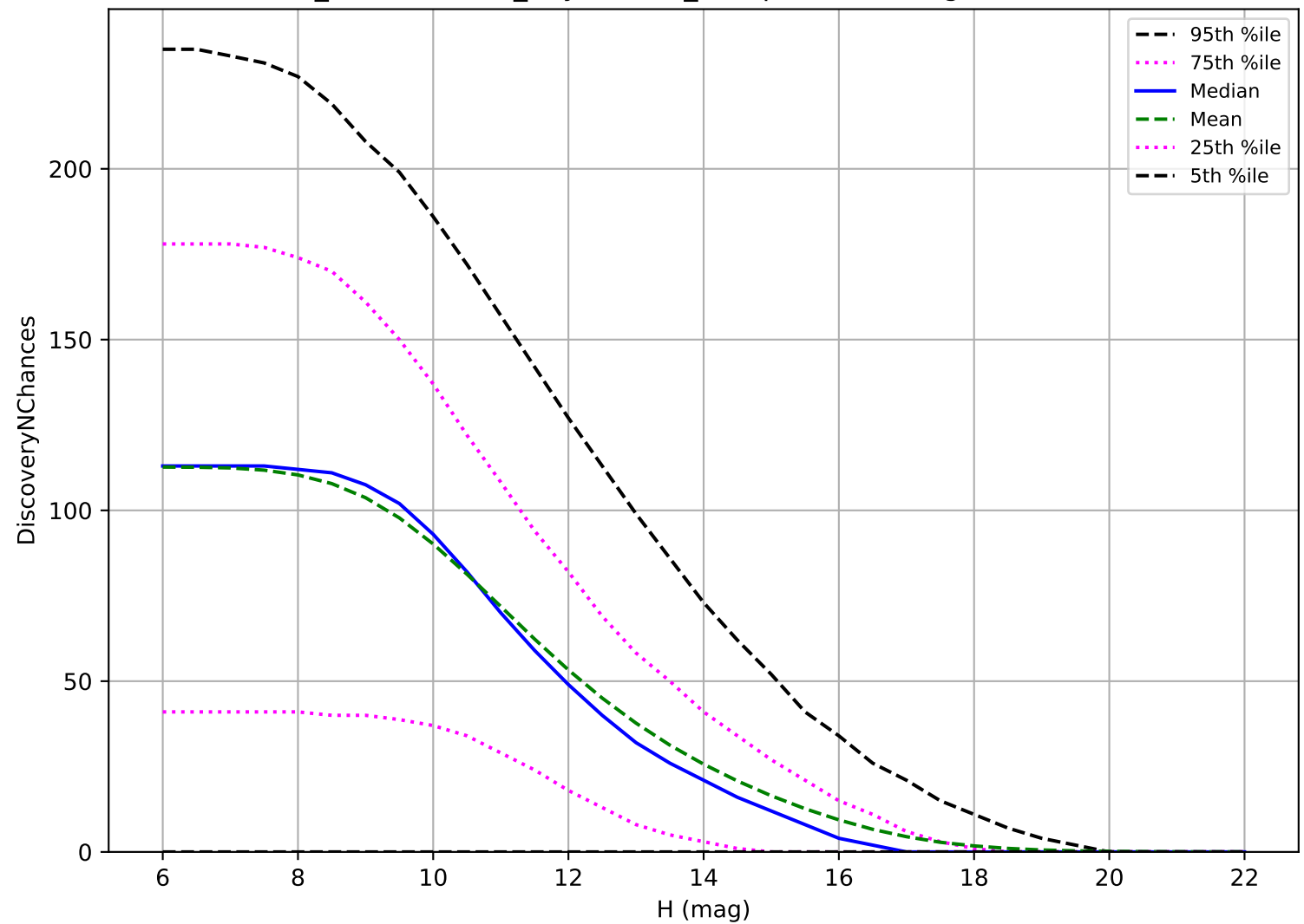
weather_cloudso4v3.4_10yrs: OCC_r5 3 pairs in 15 nights detection loss
