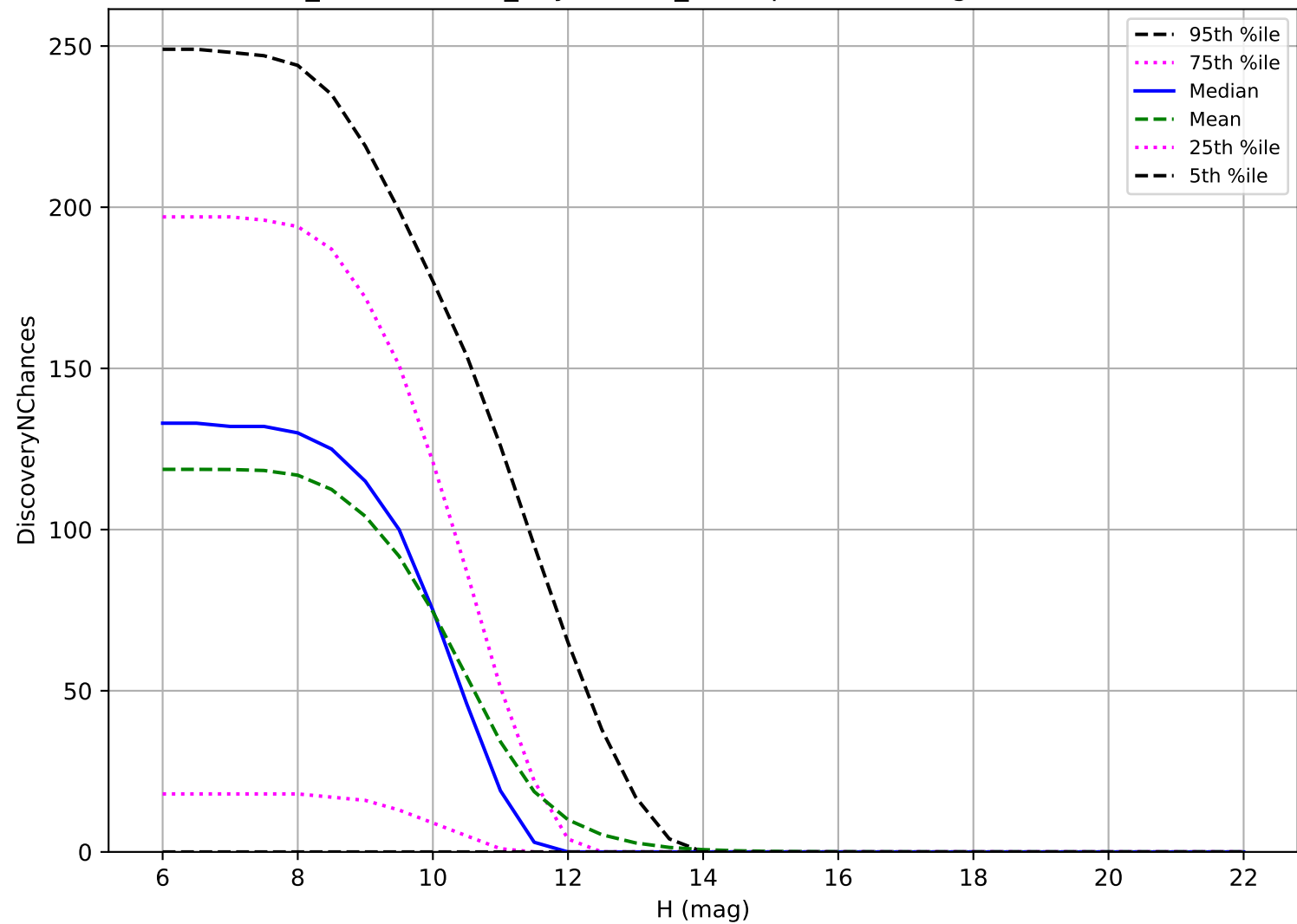
weather_cloudso4v3.4_10yrs: OCC_r20 3 pairs in 15 nights detection loss
