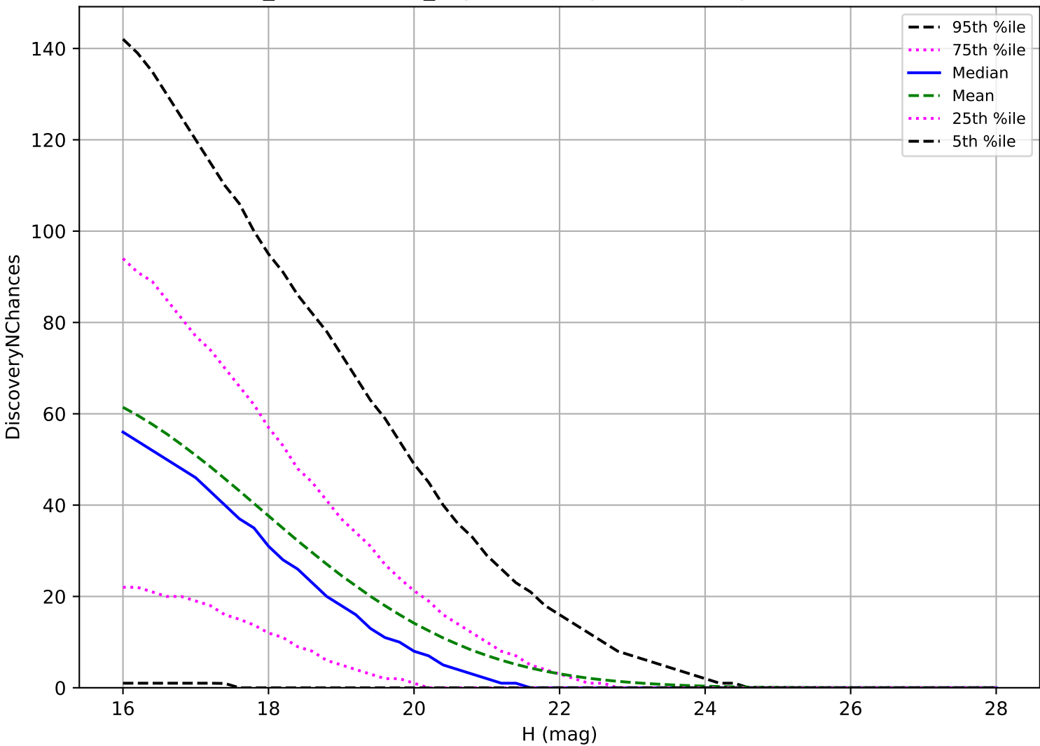
weather_cloudso4v3.4_10yrs: NEO 3 pairs in 15 nights detection loss
