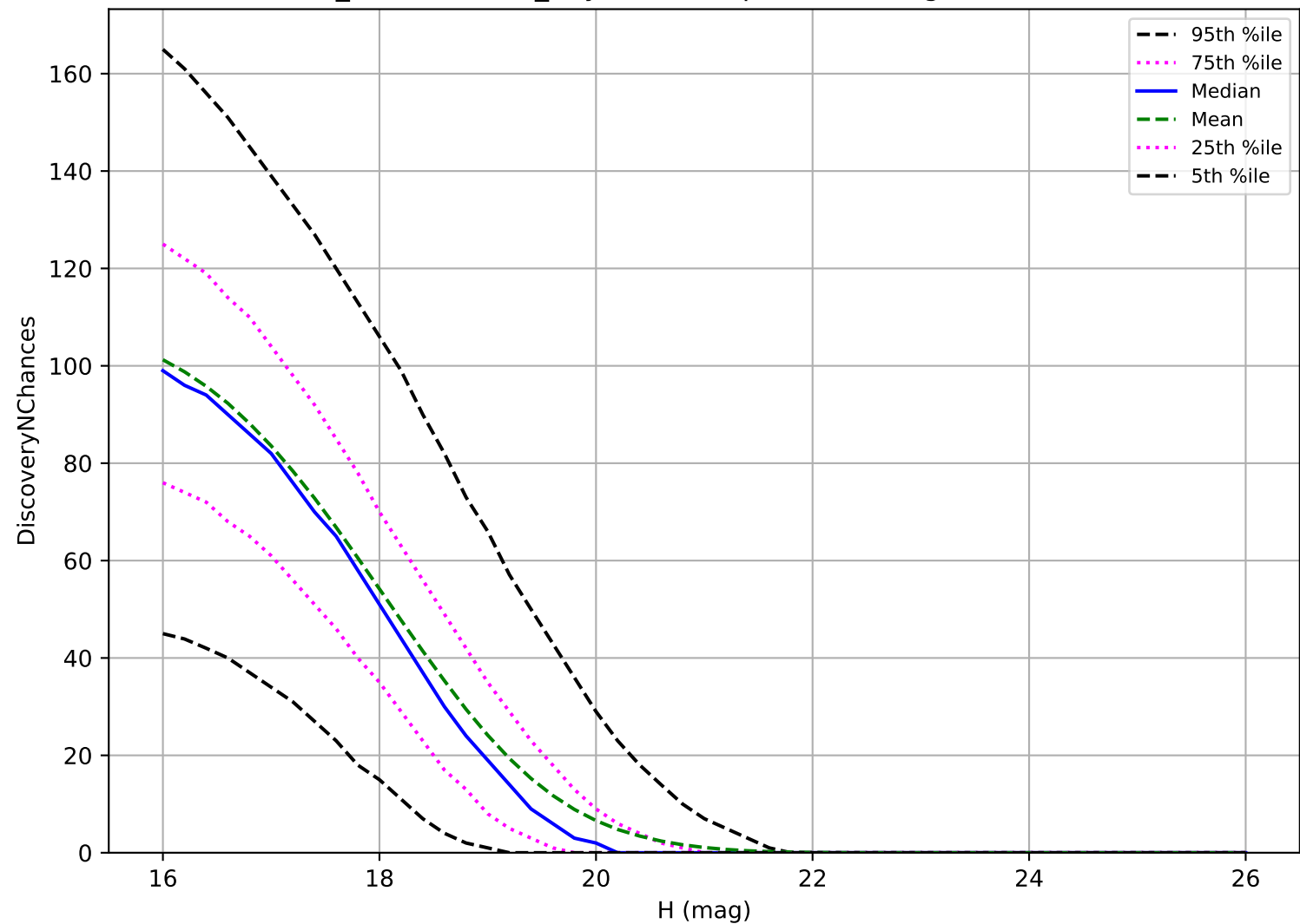
weather_cloudso4v3.4_10yrs: MBA 3 pairs in 15 nights detection loss
