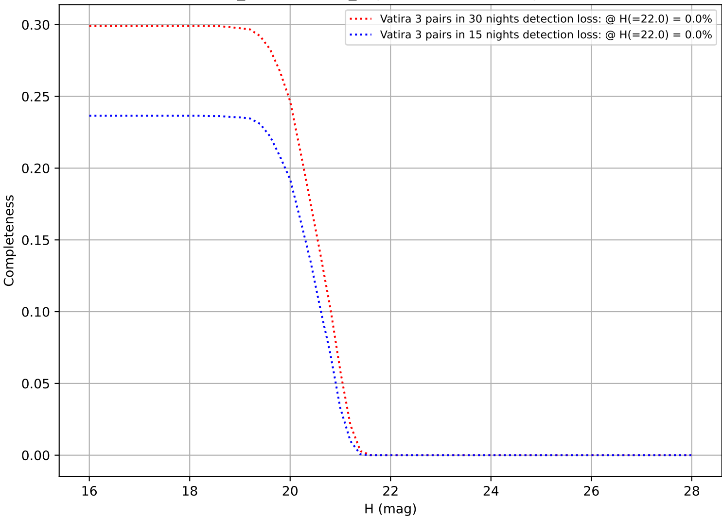
weather_cloudso4v3.4_10yrs: DifferentialCompleteness
