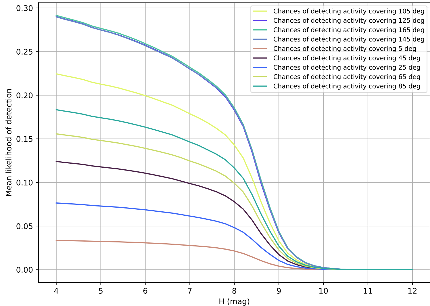
weather_cloudso4v3.4_10yrs TNO
