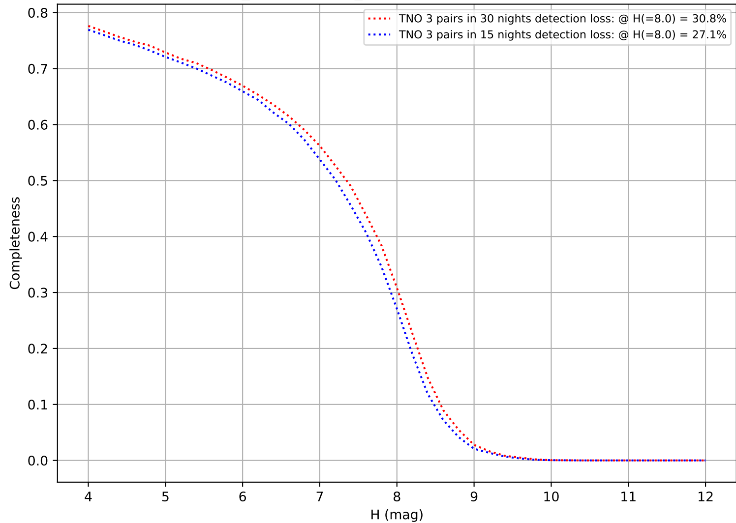
weather_cloudso4v3.4_10yrs: DifferentialCompleteness
