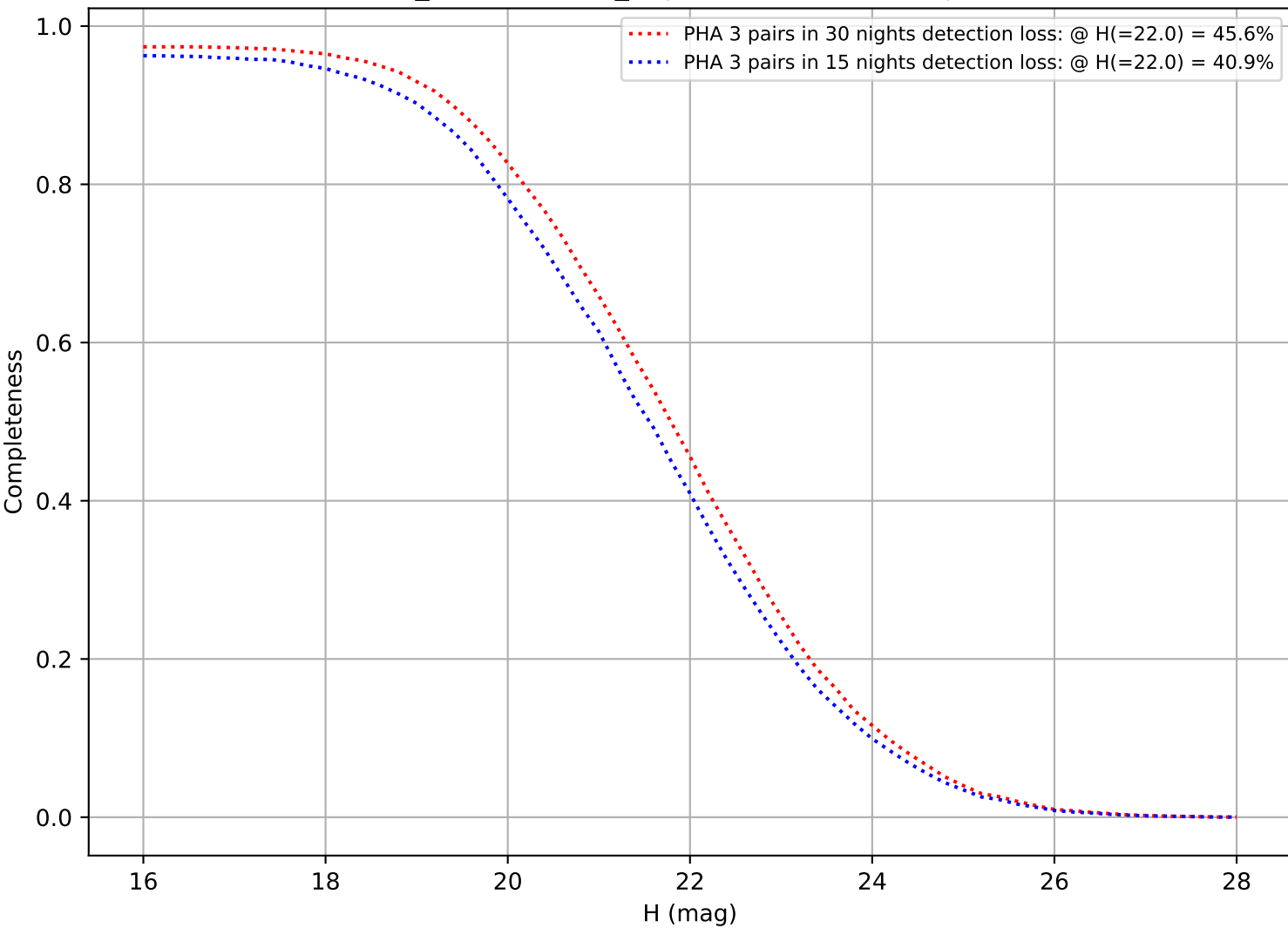
weather_cloudso4v3.4_10yrs: DifferentialCompleteness
