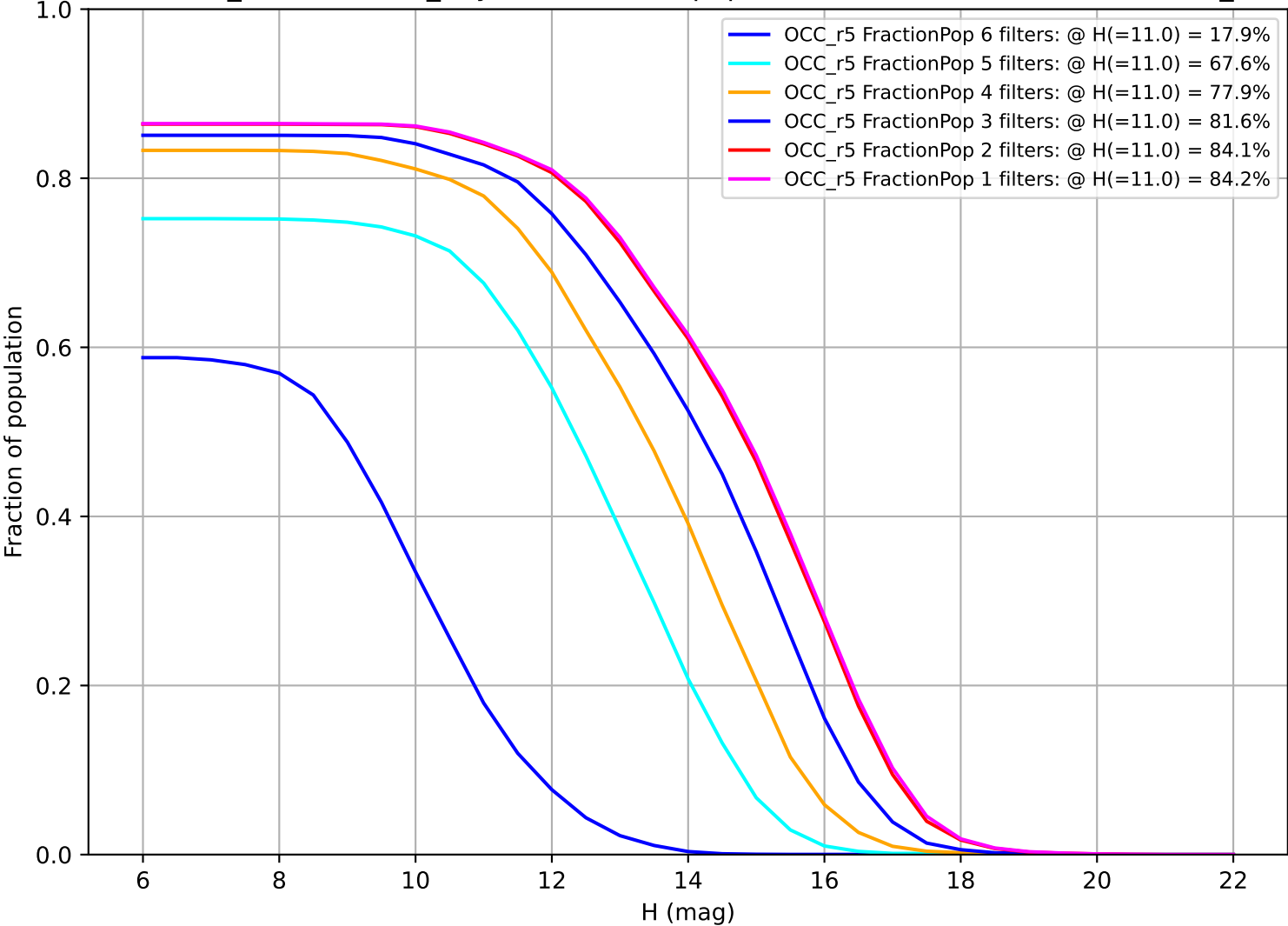
weather_cloudso4v3.4_10yrs: Fraction of population with colors in X filters OCC_r5
