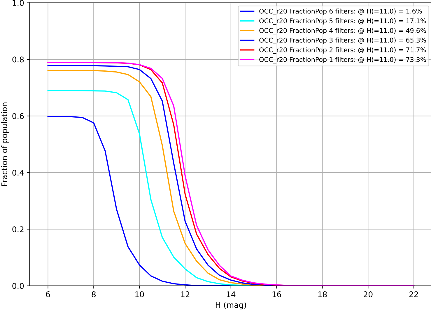
weather_cloudso4v3.4_10yrs: Fraction of population with colors in X filters OCC_r20
