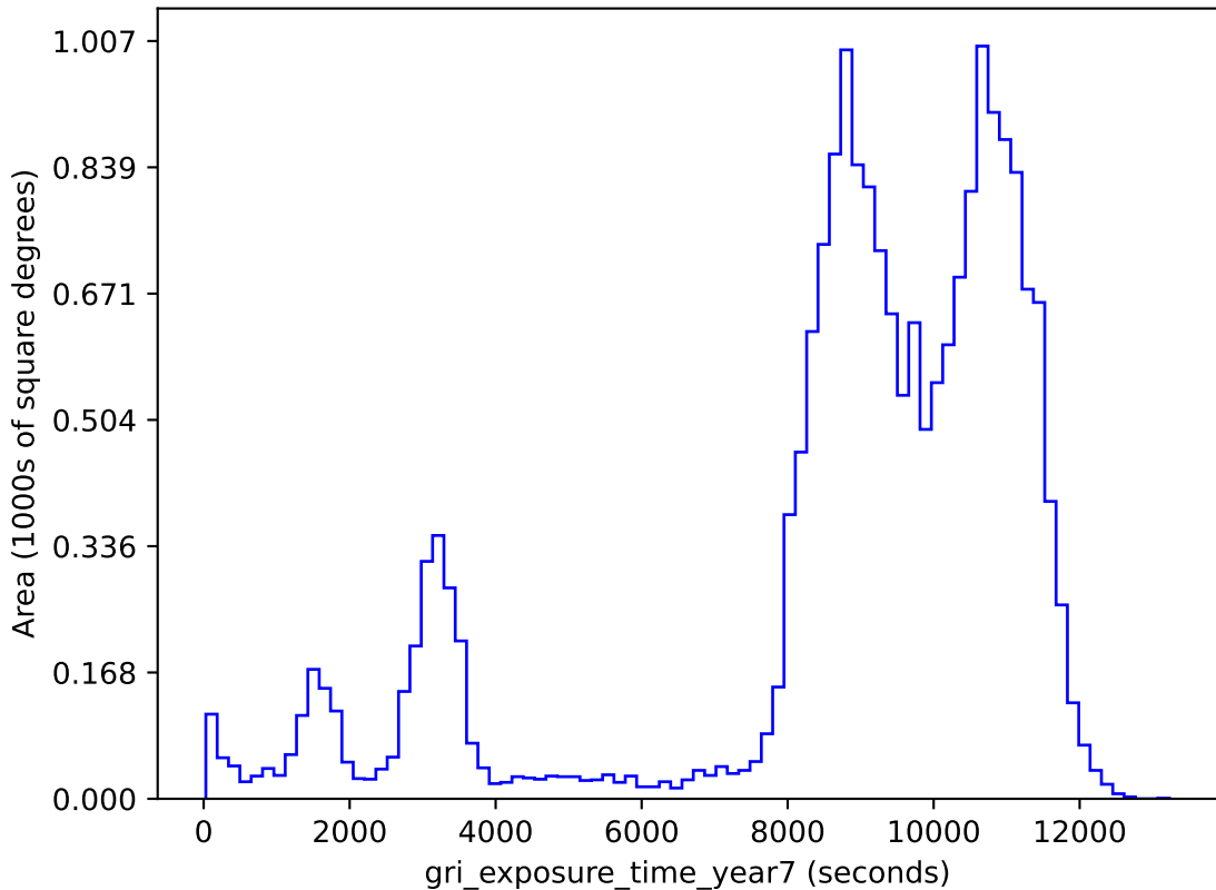
weather_cloudso4v3.4_10yrs gri band non-DD: gri_exposure_time_year7
