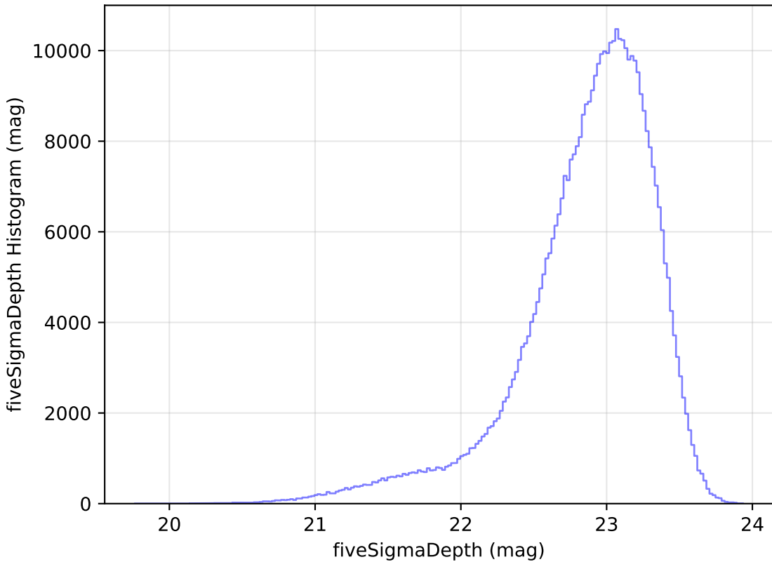
weather_cloudso4v3.4_10yrs z: fiveSigmaDepth Histogram
