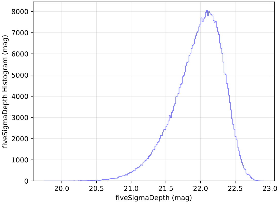
weather_cloudso4v3.4_10yrs y: fiveSigmaDepth Histogram
