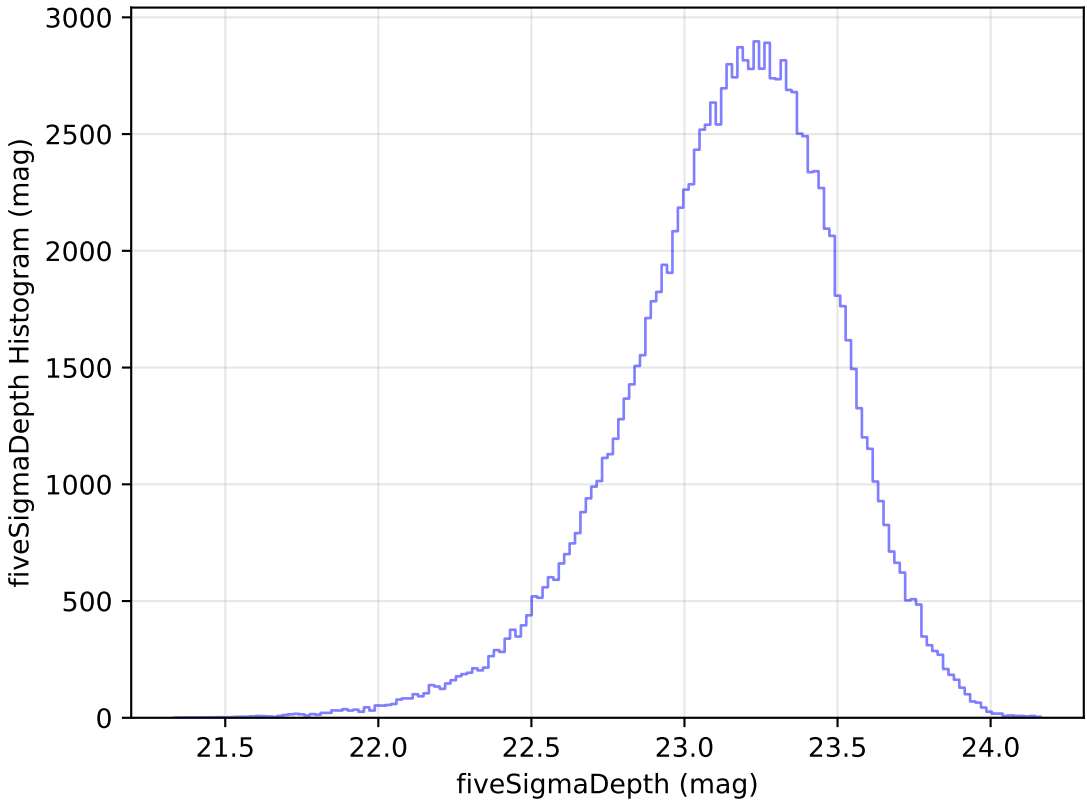
weather_cloudso4v3.4_10yrs u: fiveSigmaDepth Histogram
