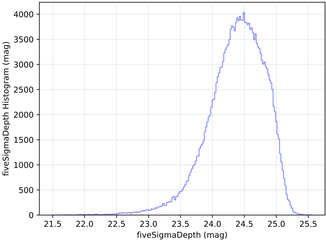
weather_cloudso4v3.4_10yrs g: fiveSigmaDepth Histogram
