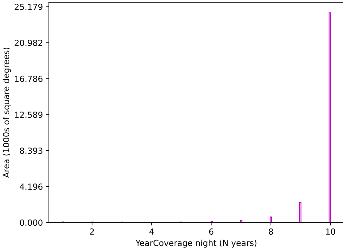
weather_cloudso4v3.4_10yrs z band: YearCoverage night
