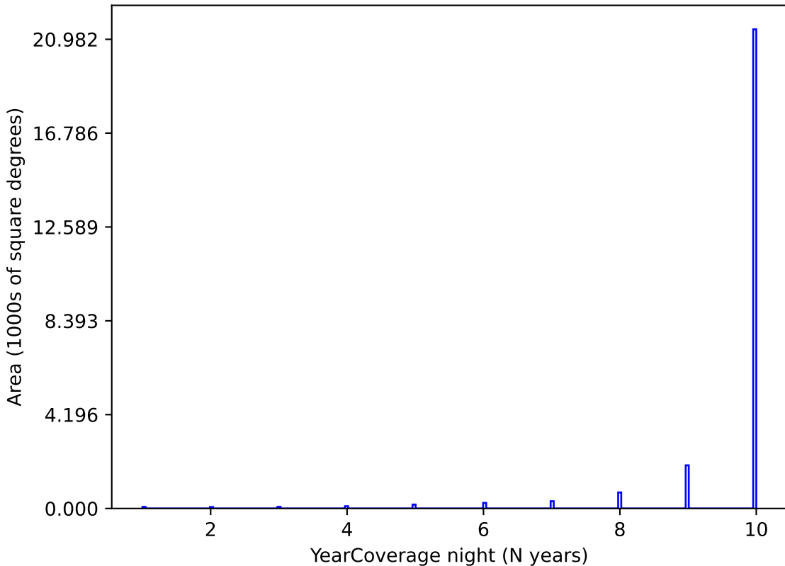
weather_cloudso4v3.4_10yrs y band: YearCoverage night
