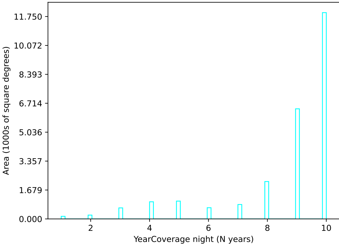
weather_cloudso4v3.4_10yrs u band: YearCoverage night
