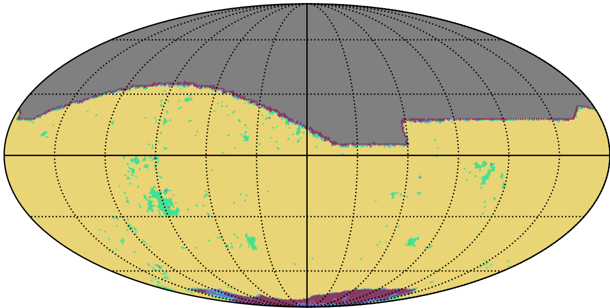
weather_cloudso4v3.4_10yrs r band: YearCoverage night
