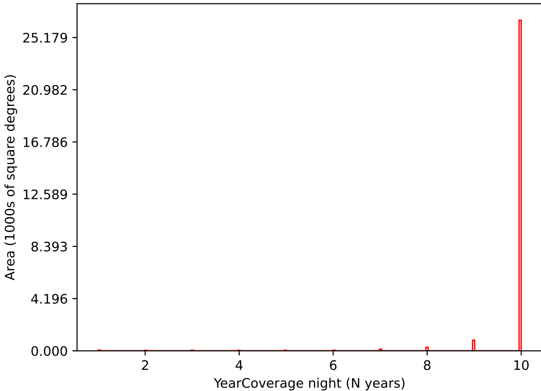
weather_cloudso4v3.4_10yrs i band: YearCoverage night
