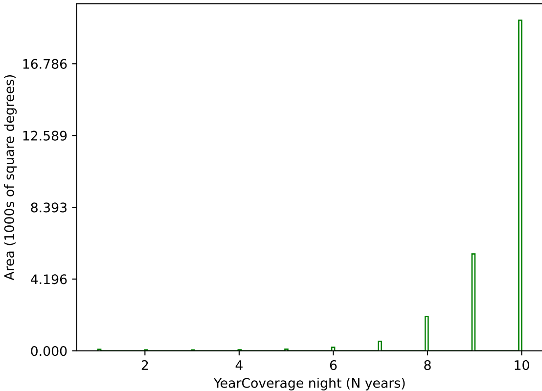
weather_cloudso4v3.4_10yrs g band: YearCoverage night
