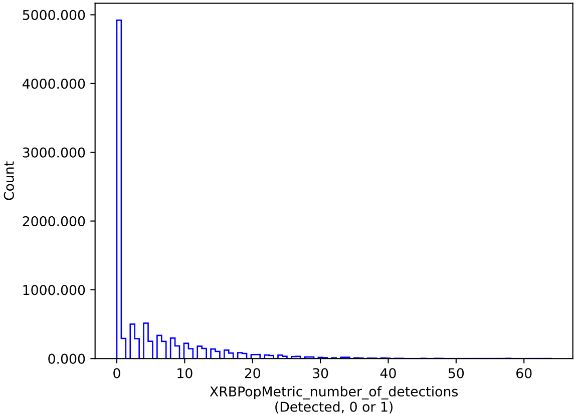
weather_cloudso4v3.4_10yrs : XRBPoMetric_number_of_detections
