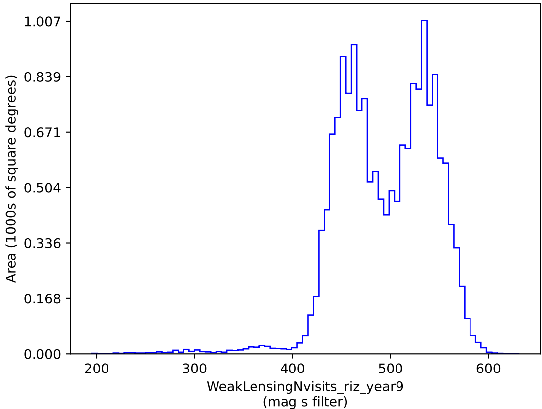
weather_cloudso4v3.4_10yrs gri band non-DD: WeakLensingNvisits_riz_year9
