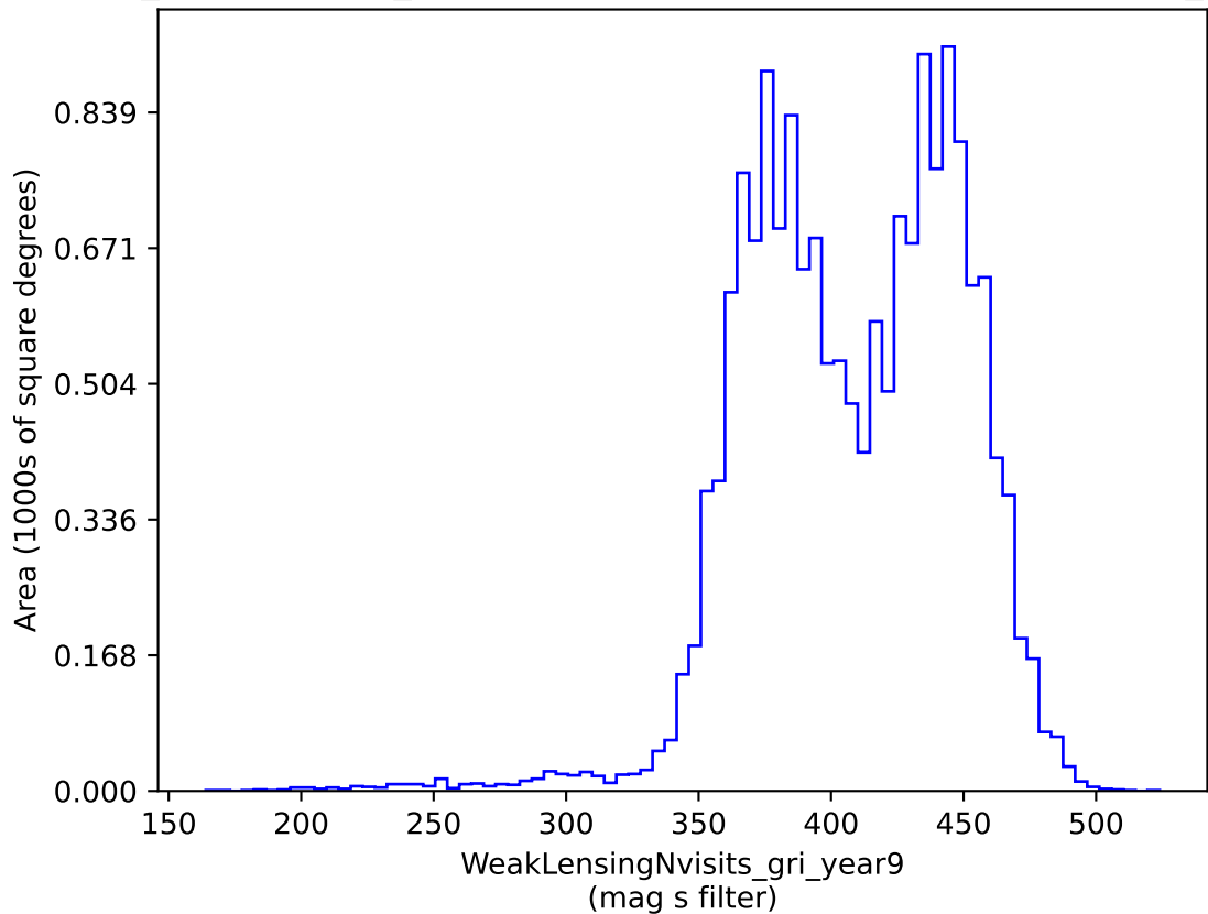
weather_cloudso4v3.4_10yrs gri band non-DD: WeakLensingNvisits_gri_year9
