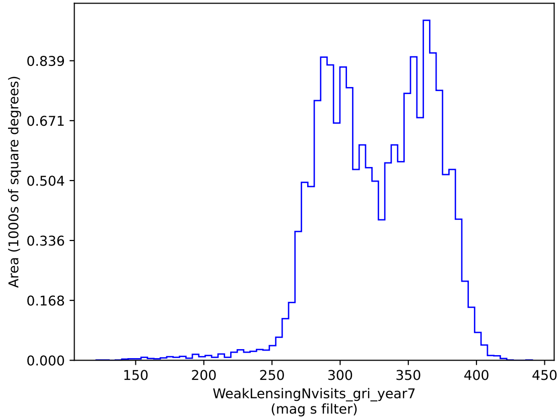
weather_cloudso4v3.4_10yrs gri band non-DD: WeakLensingNvisits_gri_year7
