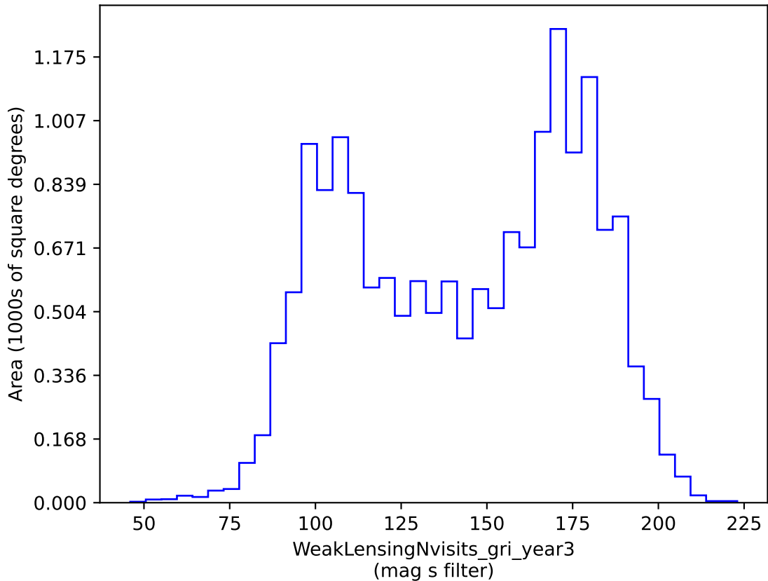
weather_cloudso4v3.4_10yrs gri band non-DD: WeakLensingNvisits_gri_year3
