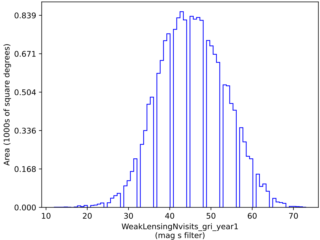
weather_cloudso4v3.4_10yrs gri band non-DD: WeakLensingNvisits_gri_year1
