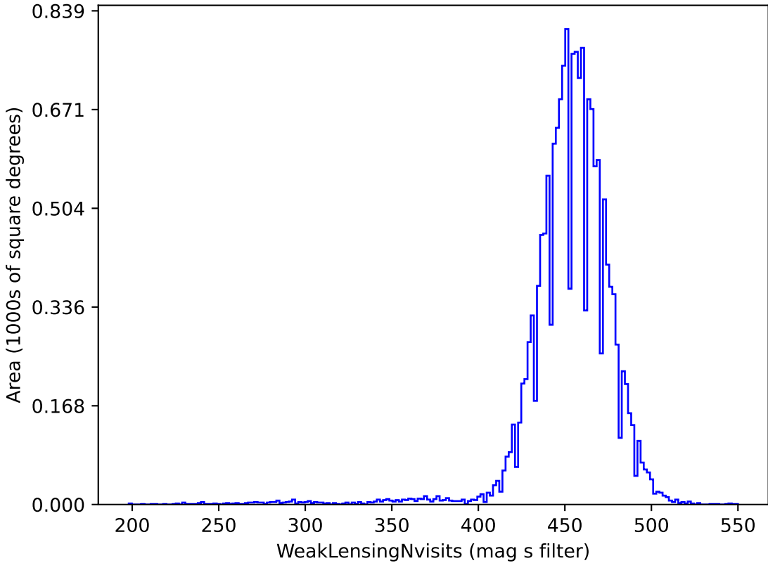
weather_cloudso4v3.4_10yrs gri band non-DD: WeakLensingNvisits
