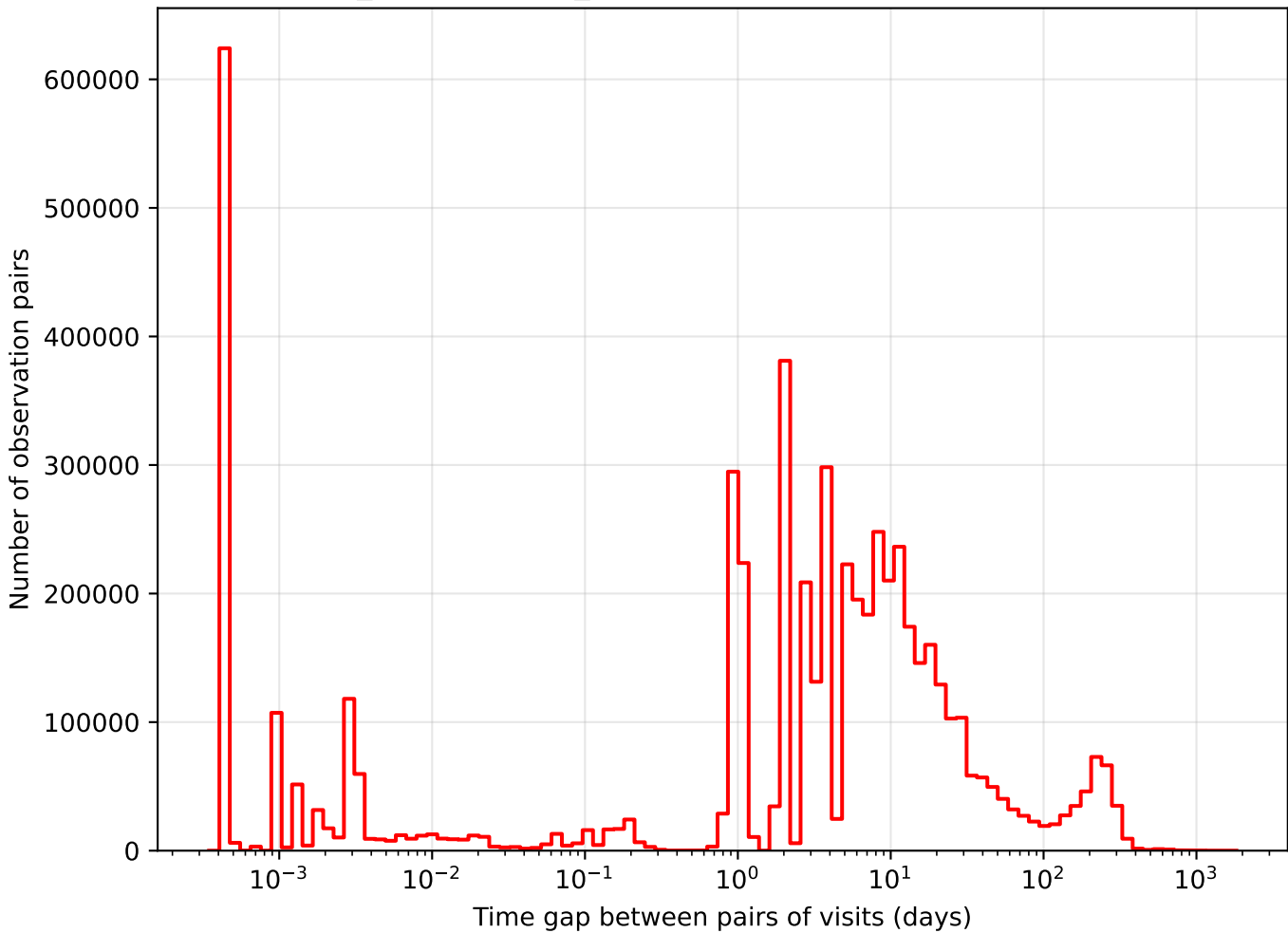
weather_cloudso4v3.4_10yrs i band: Tgaps observationStartMJD
