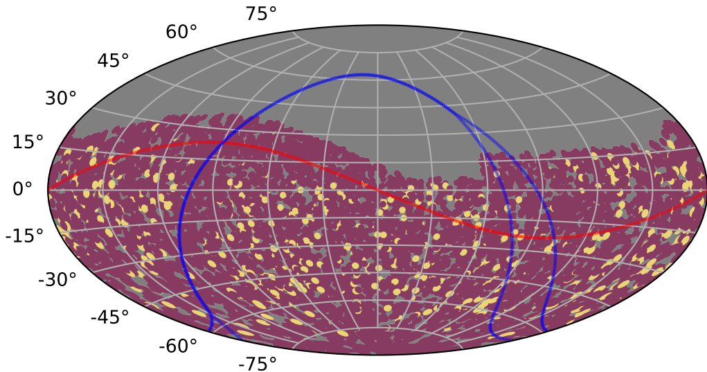
weather_cloudso4v3.4_10yrs : TDEsPopMetric_some_color
