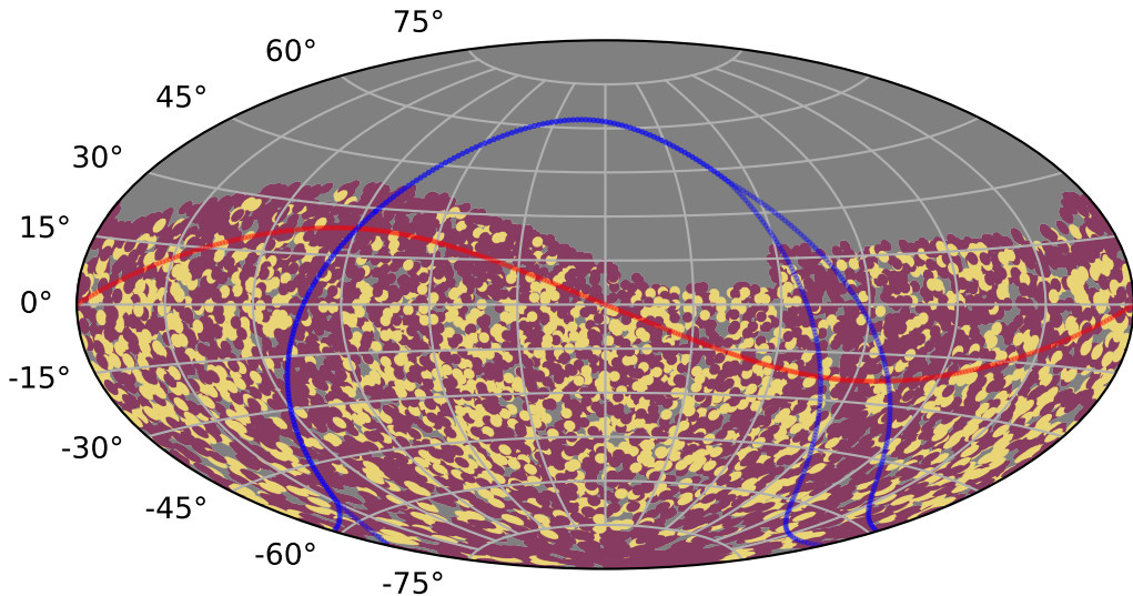
weather_cloudso4v3.4_10yrs : TDEsPopMetric_prepeak
