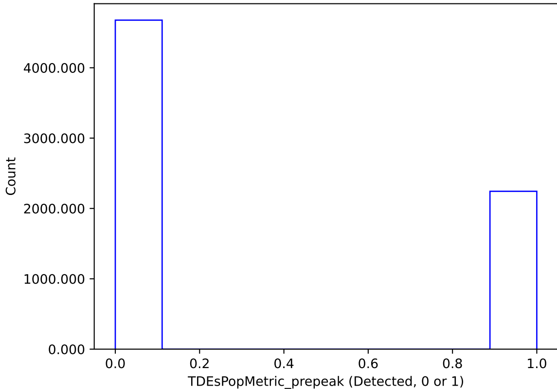
weather_cloudso4v3.4_10yrs : TDEsPopMetric_prepeak
