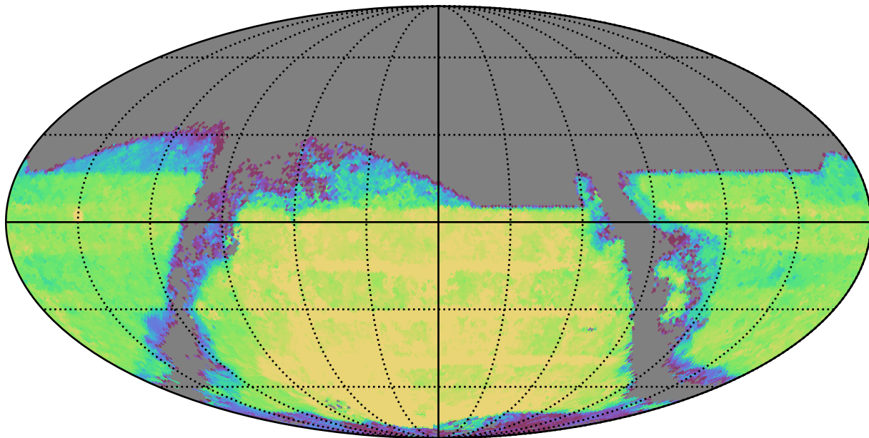
weather_cloudso4v3.4_10yrs : TDC_season
