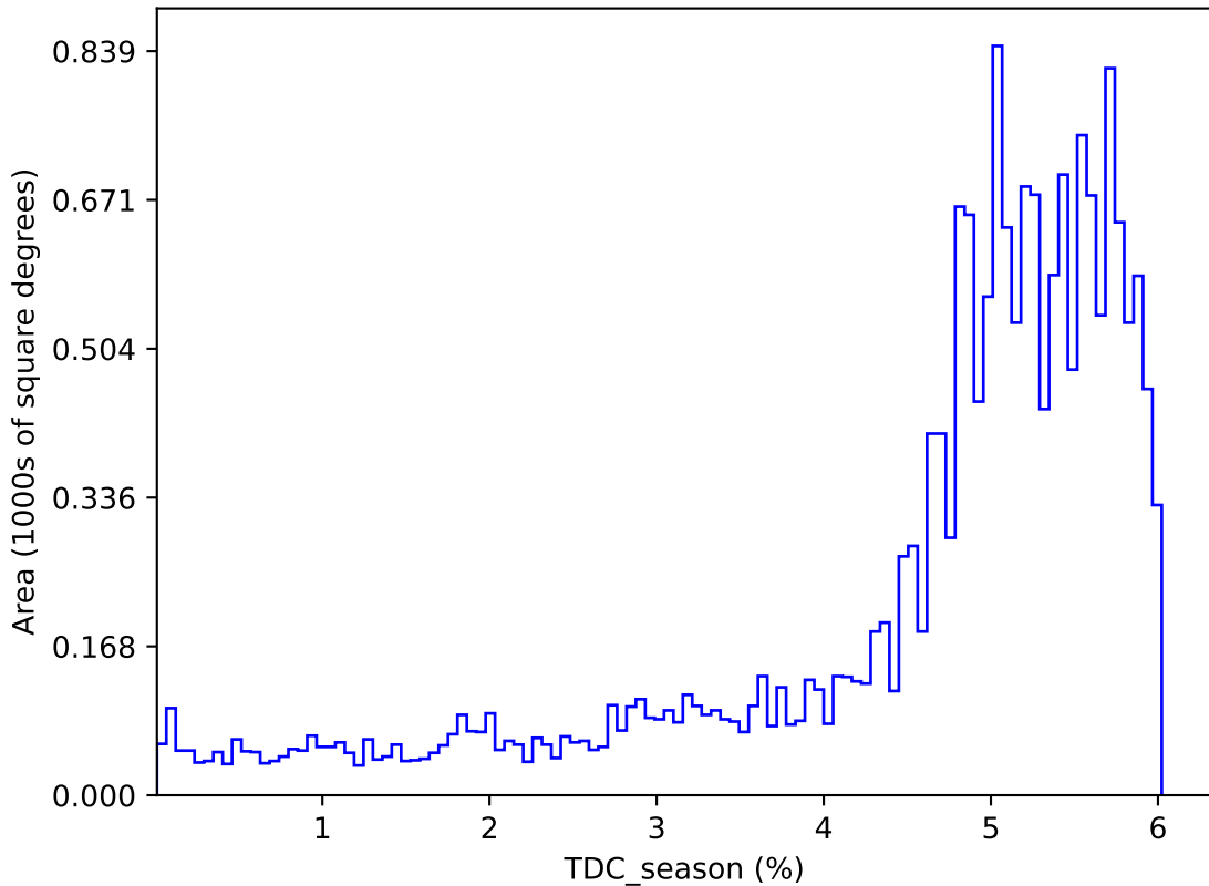
weather_cloudso4v3.4_10yrs : TDC_season
