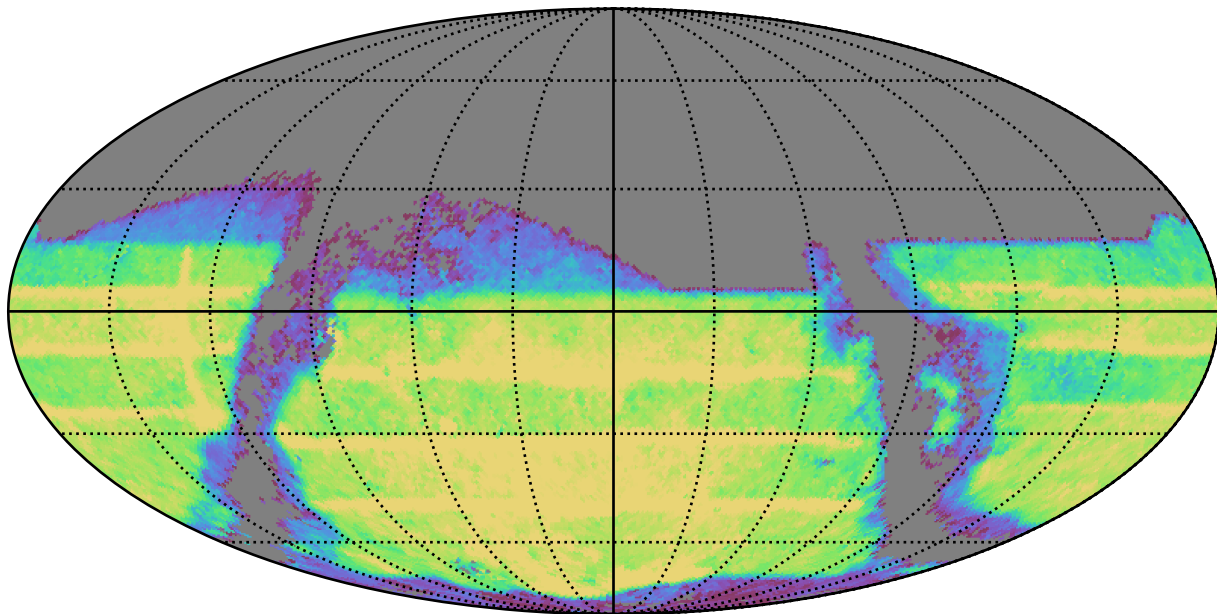
weather_cloudso4v3.4_10yrs : TDC_rate
