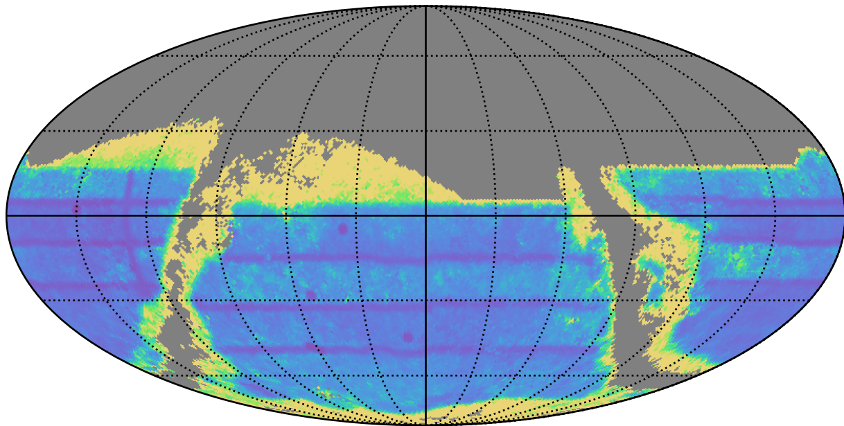
weather_cloudso4v3.4_10yrs : TDC_precision
