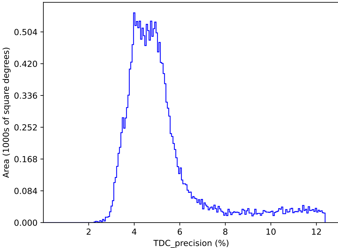
weather_cloudso4v3.4_10yrs : TDC_precision
