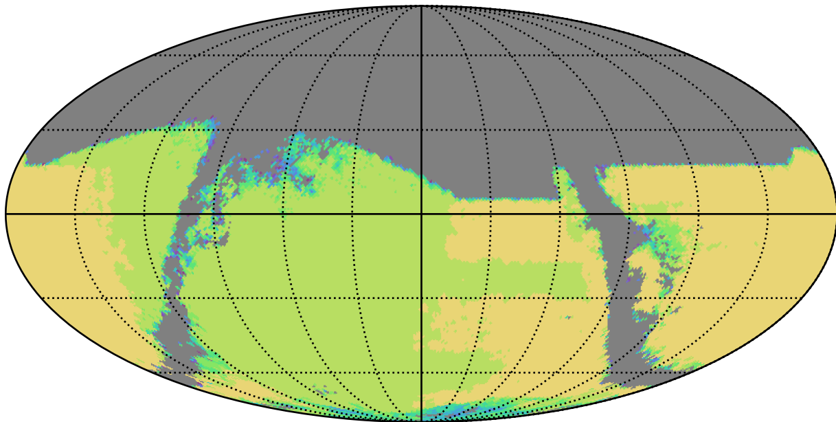
weather_cloudso4v3.4_10yrs : TDC_campaign
