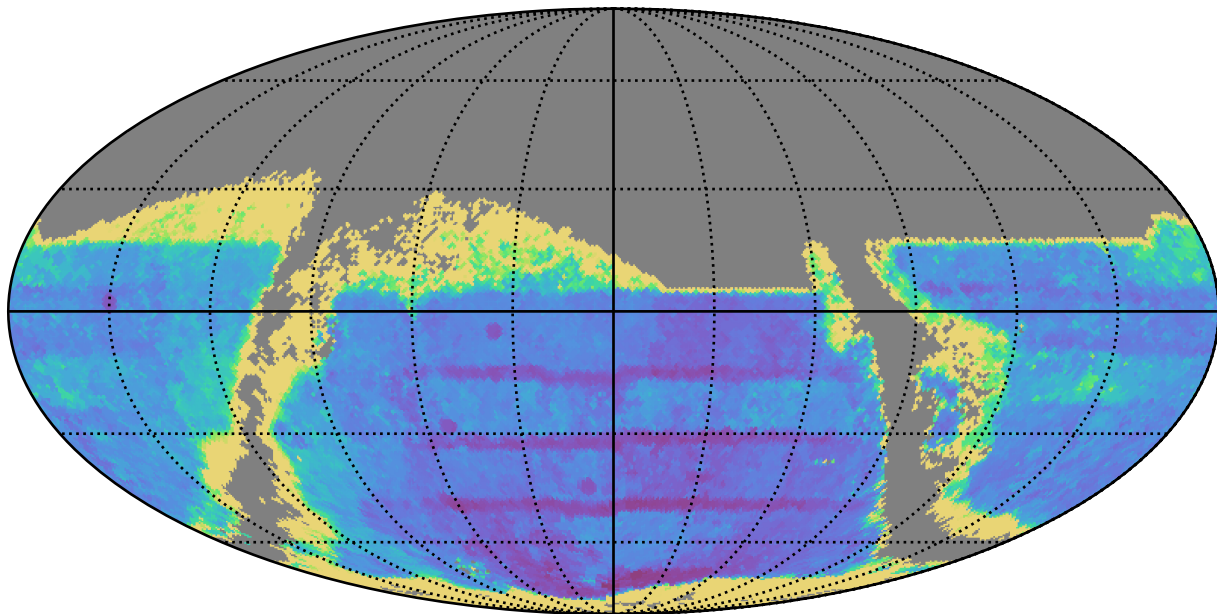
weather_cloudso4v3.4_10yrs : TDC_accuracy
