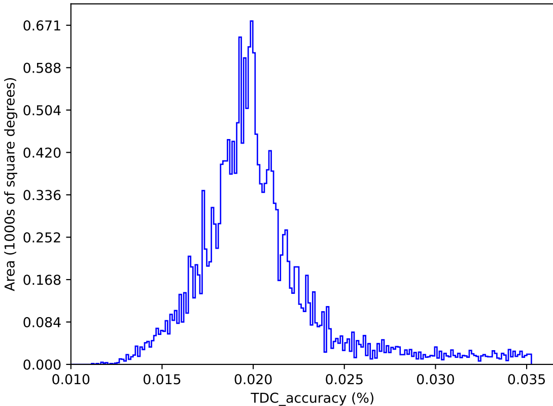
weather_cloudso4v3.4_10yrs : TDC_accuracy
