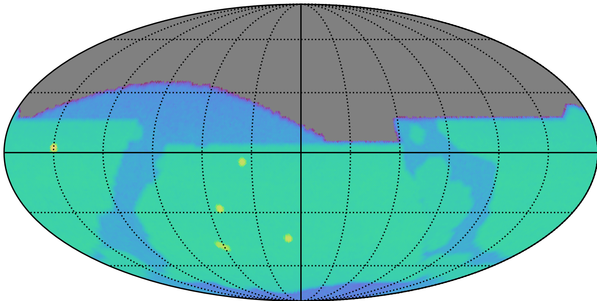
weather_cloudso4v3.4_10yrs z: SurfaceBrightLimit
