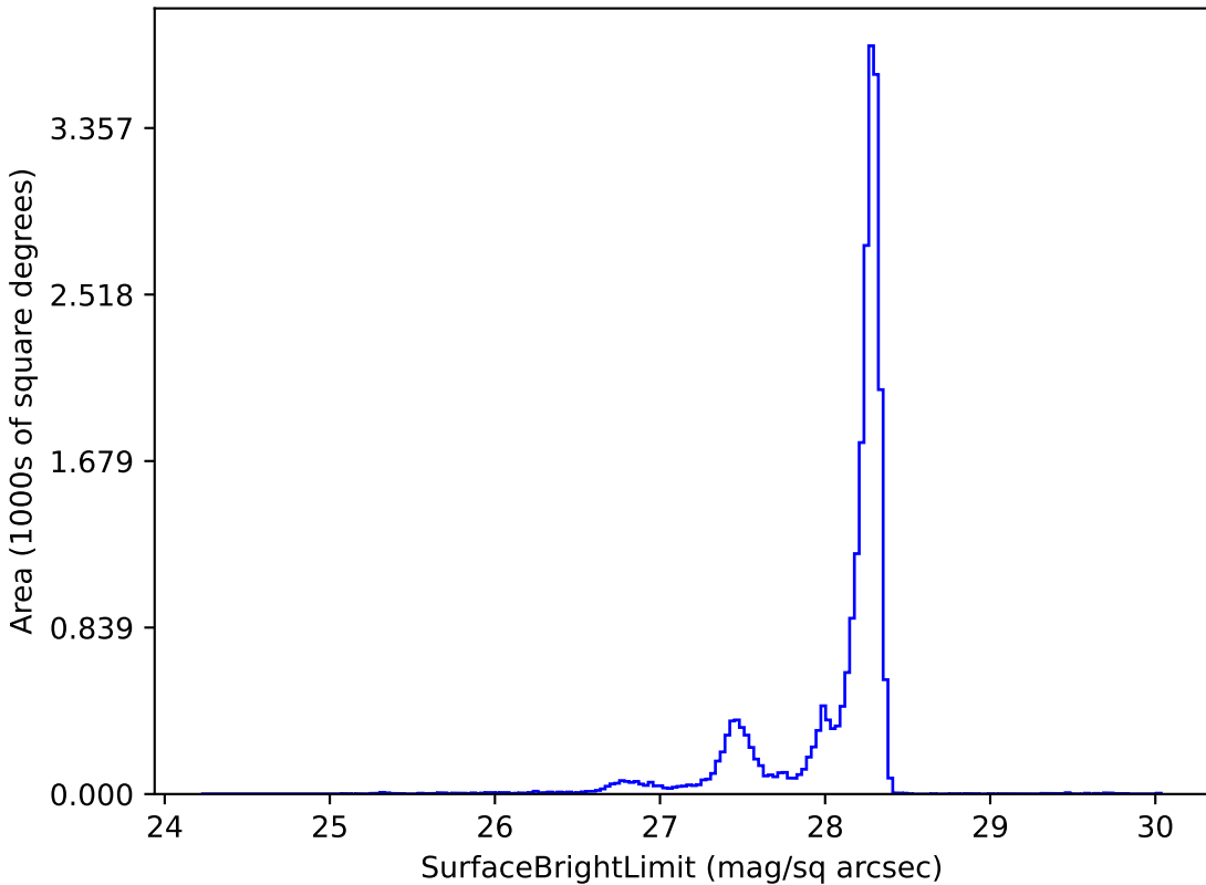
weather_cloudso4v3.4_10yrs y: SurfaceBrightLimit
