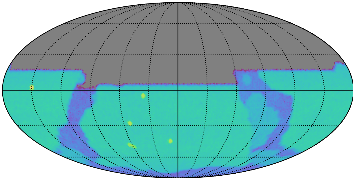
weather_cloudso4v3.4_10yrs u: SurfaceBrightLimit
