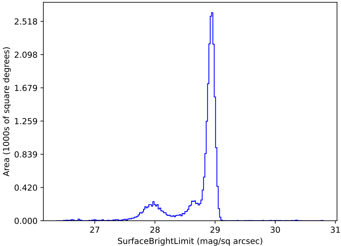
weather_cloudso4v3.4_10yrs u: SurfaceBrightLimit
