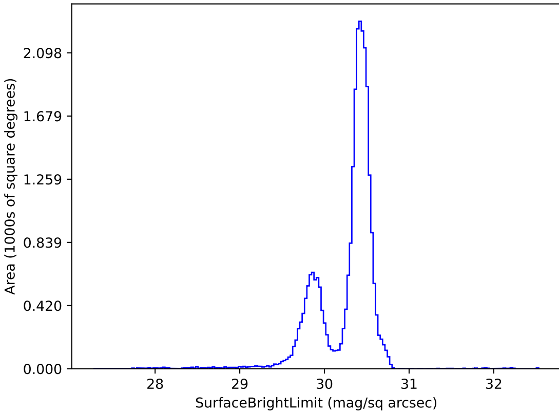
weather_cloudso4v3.4_10yrs g: SurfaceBrightLimit
